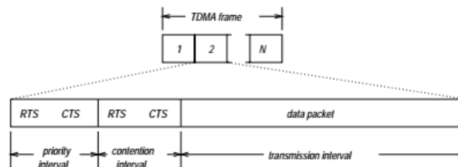
Fig. 1.13 The ADAPT protocol.
