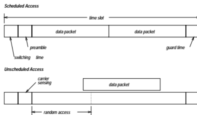
Fig. 1.12 Hybrid TDMA/CSMA channel access.
