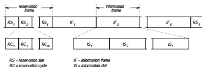
Fig. 1.11 Frame and slot structure of FPRP.
